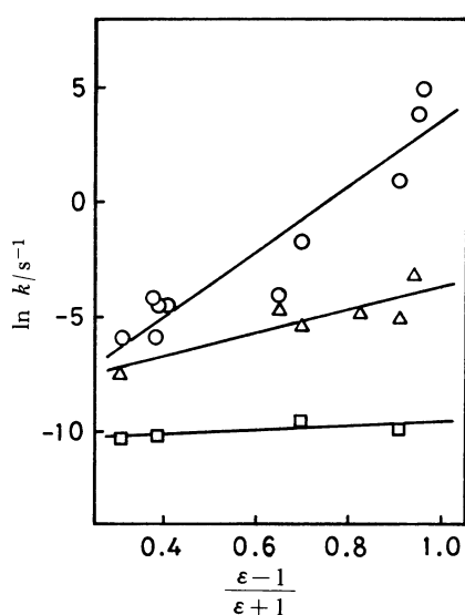
Fig. 2. Plots of \ln k against (\epsilon-1)/(\epsilon+1) , according to Eq. 4: (O) NDAAB; ( \Delta ) BDEAAB; ( \square ) DAAB.
